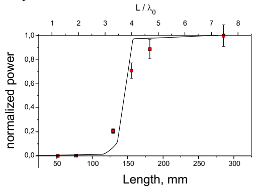
Figure 4: Dependence of electromagnetic radiation on L for experimental setup [13]
