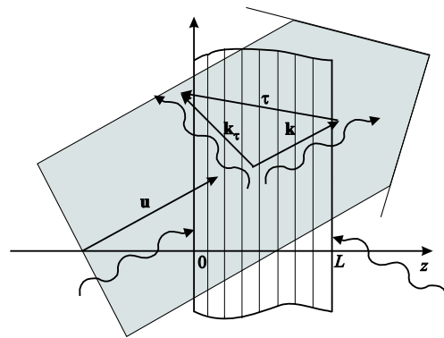
Figure 1: Scheme of two-wave VFEL in Bragg geometry.
