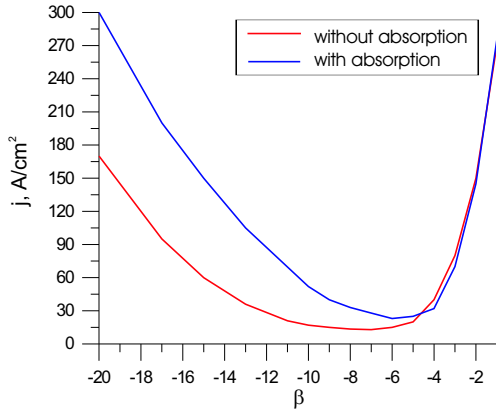
Figure 2: Dependence of the threshold current on asymmetry factor of VDFB
