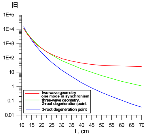
Figure 3: Current threshold for two- and three-wave geometry in dependence on L
